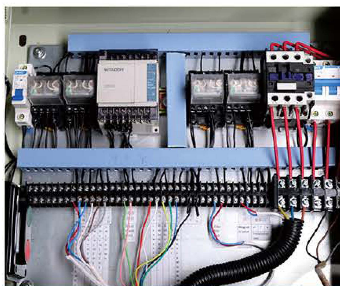
PLC control system
